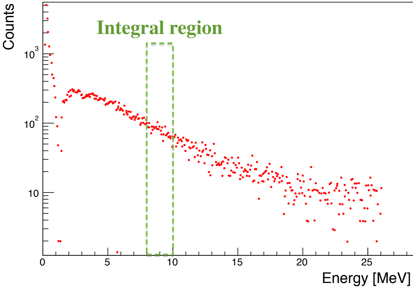
Reproduced charged particle spectrum by Sobottka et al.
