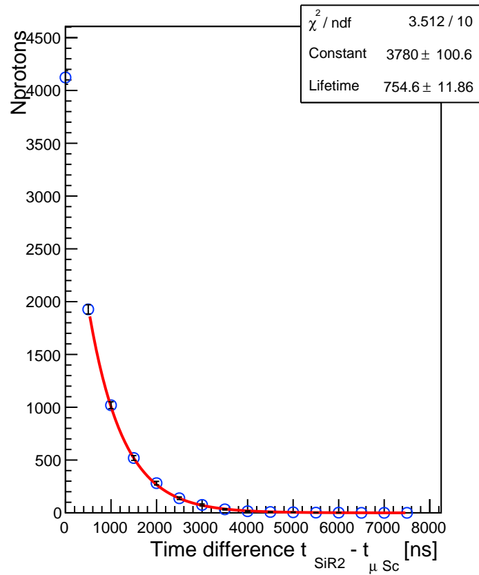
Number of protons from Si16p with time cuts - Right
