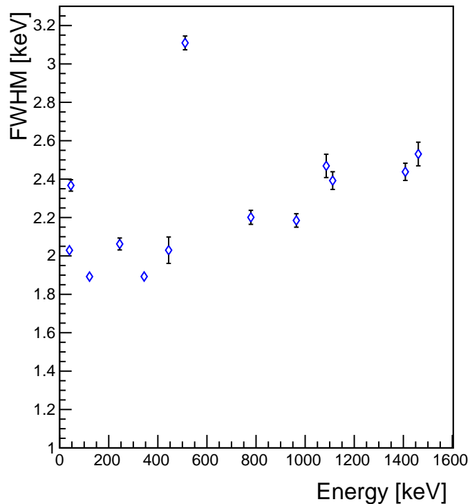
Resolution (FWHM)
