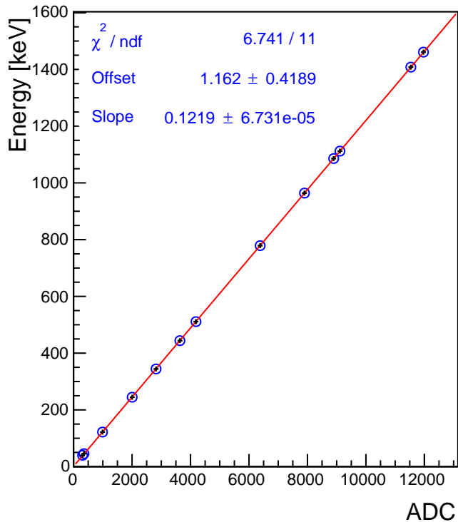
Energy calibration for germanium detector
