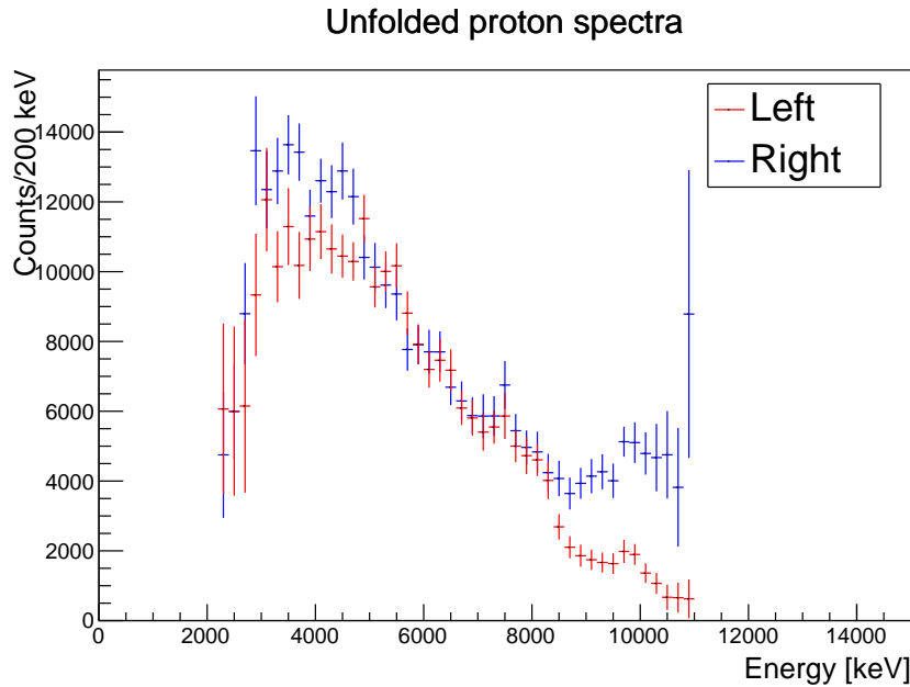
Figure 5.11: Unfolded proton spectra from the 100- \mu m aluminium target.
