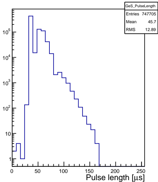
Germanium - Pulse length
