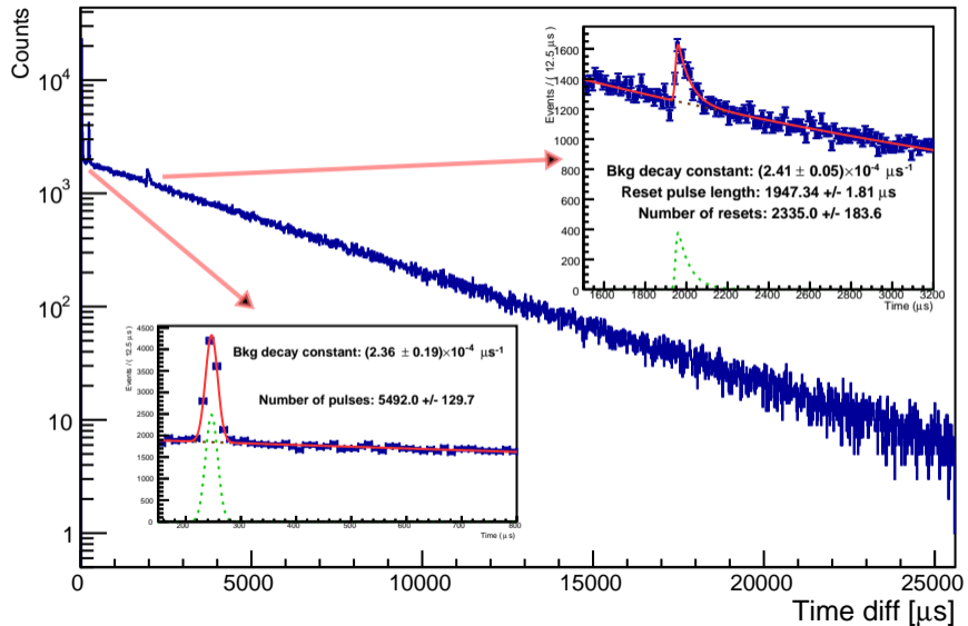
Germanium - Interval between two consecutive pulses
