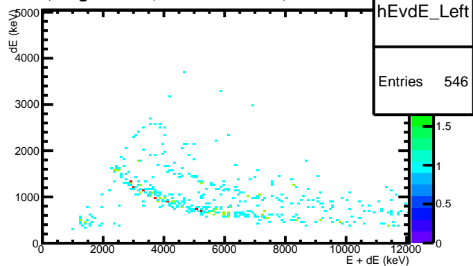
dEdx, target Al100, runs 2840-2851, left
