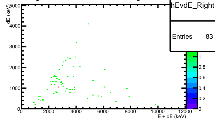
dEdx, target Al100, runs 2840-2851, right
