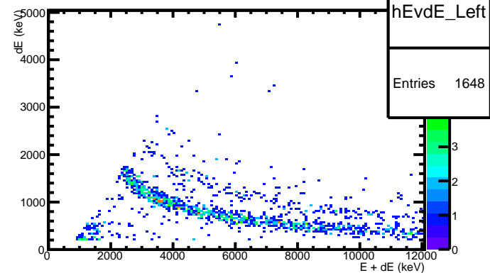
dEdx, target Si16_passive, runs 3474-3500, left
